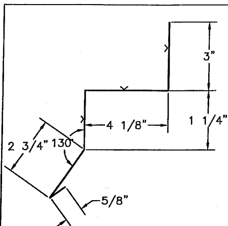
ULTRA GLIDE TOP MOUNT TRACK COVER
