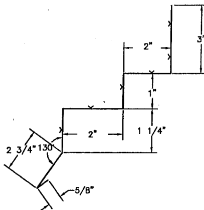
ULTRA GLIDE FACE MOUNT TRACK COVER
