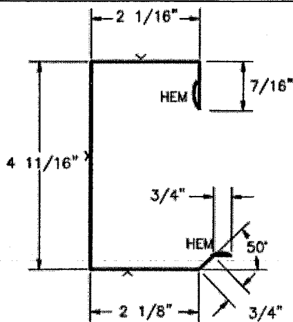
Vertical Frame Cover
