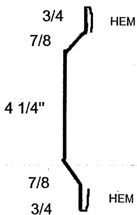
Double Frame Cover
