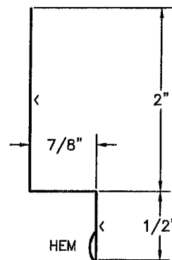
BOTTOM DOOR TRIM (WAINSCOT TRANSITION)
